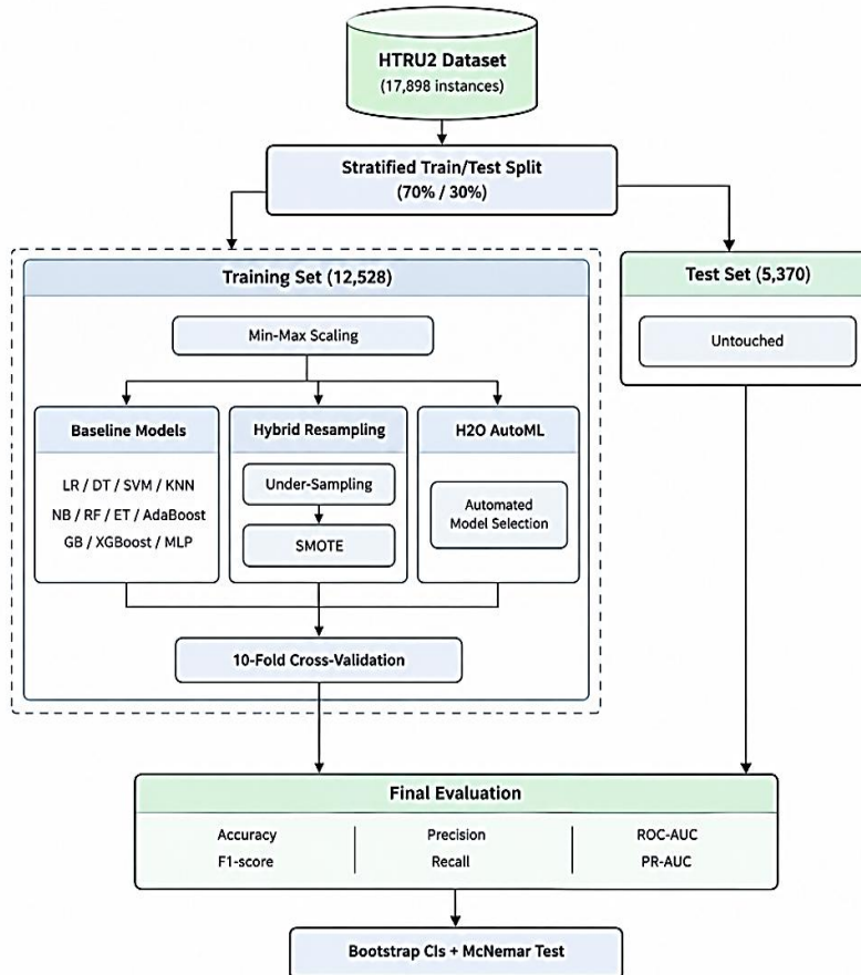
Fig. 1. :Overall leakage-free comparative framework.
