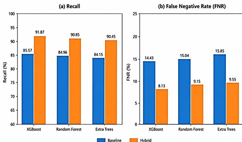
Fig. 4. Recall and False Negative Rate (FNR) before and after hybrid resampling for XGBoost, Random Forest, and Extra Trees.
