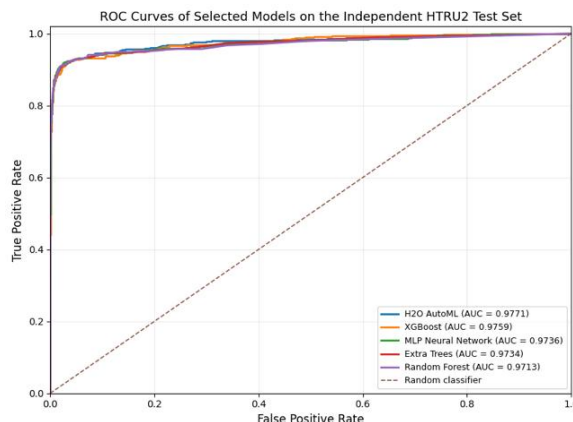
Fig. 3. ROC curves of selected models on the independent HTRU2 test set.
